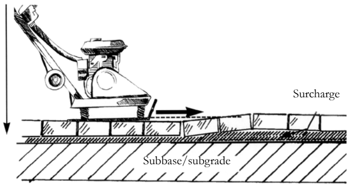
Using a vibrator to compact the pavement
