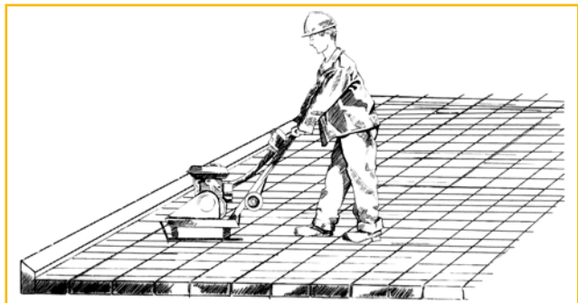
Figure 16: Vibrating the blocks into the bedding sand layer
