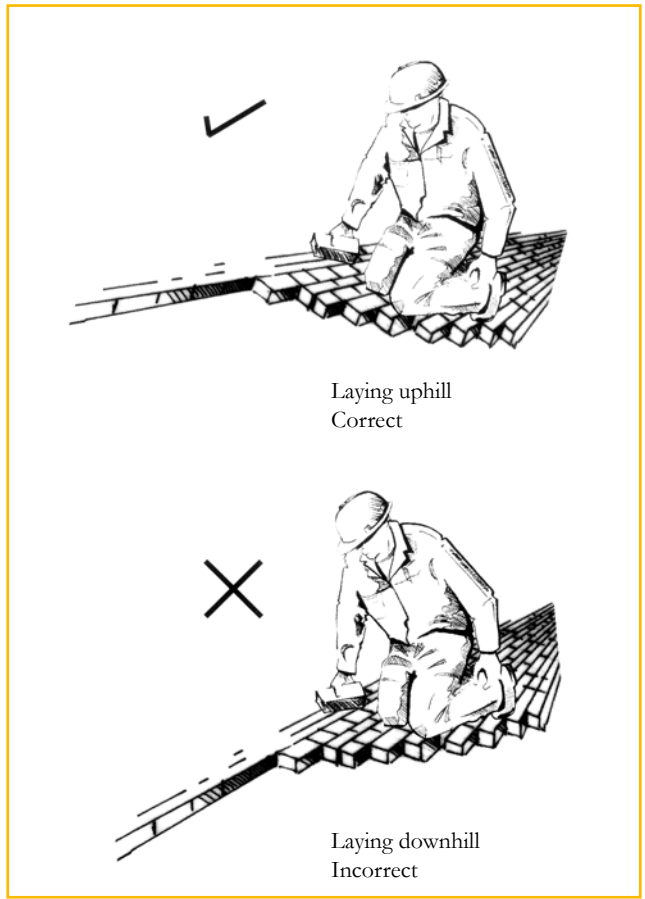
Figure 10: Laying on an incline
