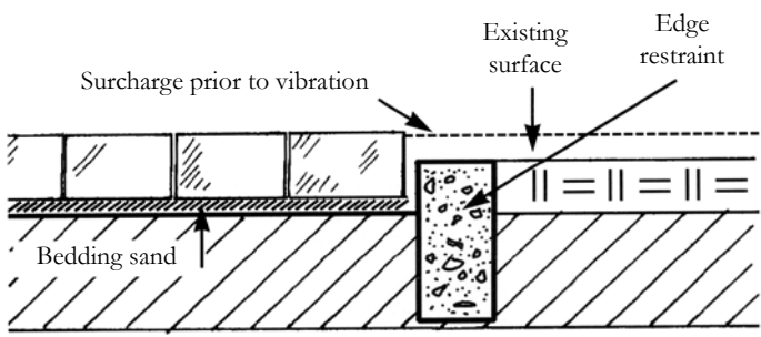
Allowing surcharge for compaction
