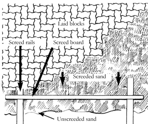
Figure 5c: Lay screeding rails approximately 2m apart
