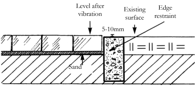
Correct levels after compaction
